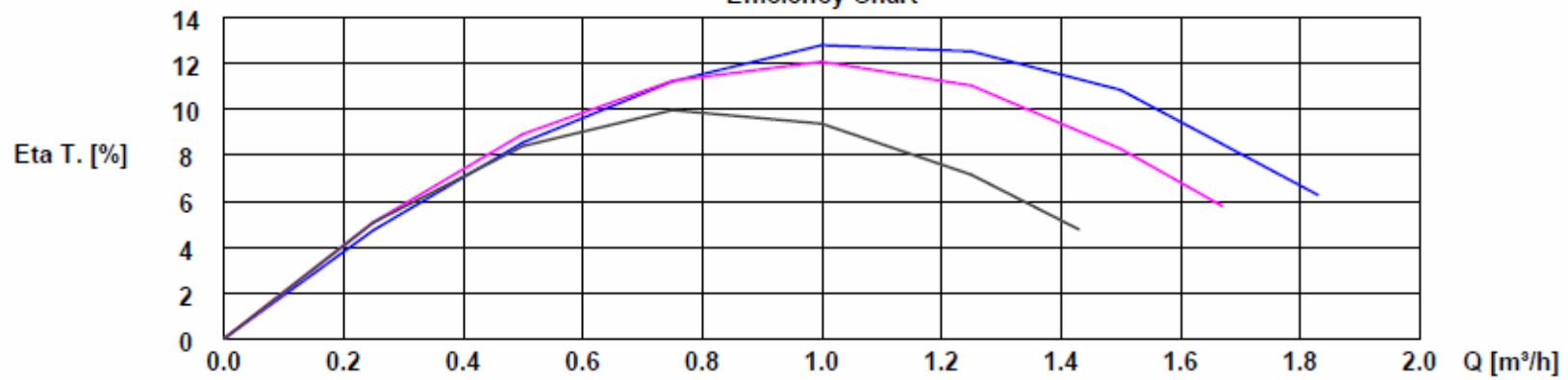
Efficiency Chart
