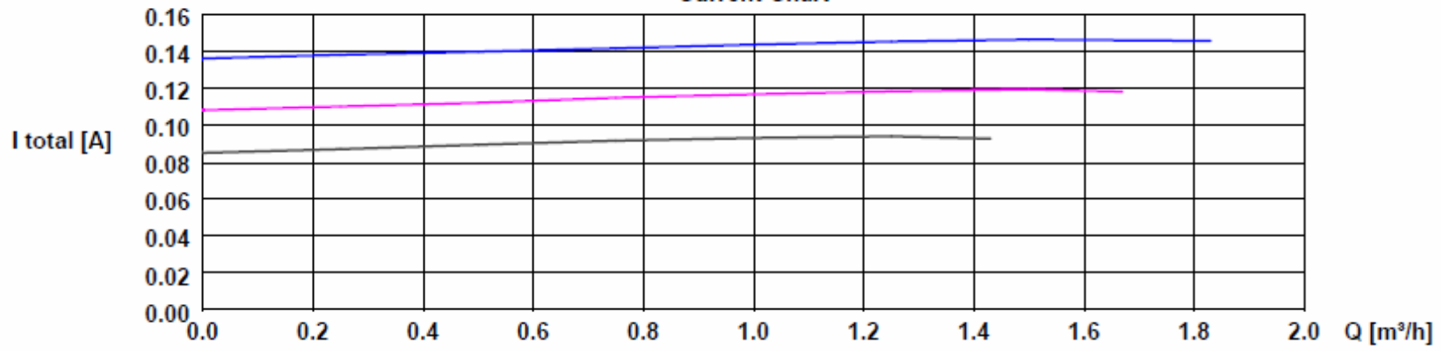
Current Chart
